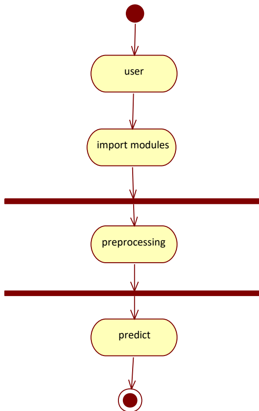
Fig.1. DFD Diagram
