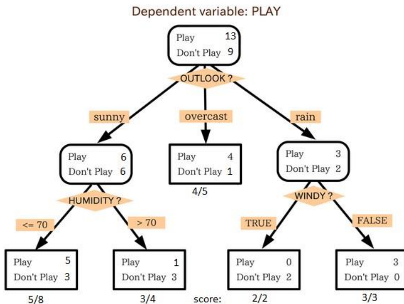
Fig.6. Decision Tree of Dependent Variable
