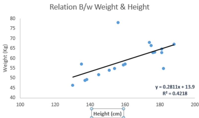
Fig.5. Linear regression Analysis
