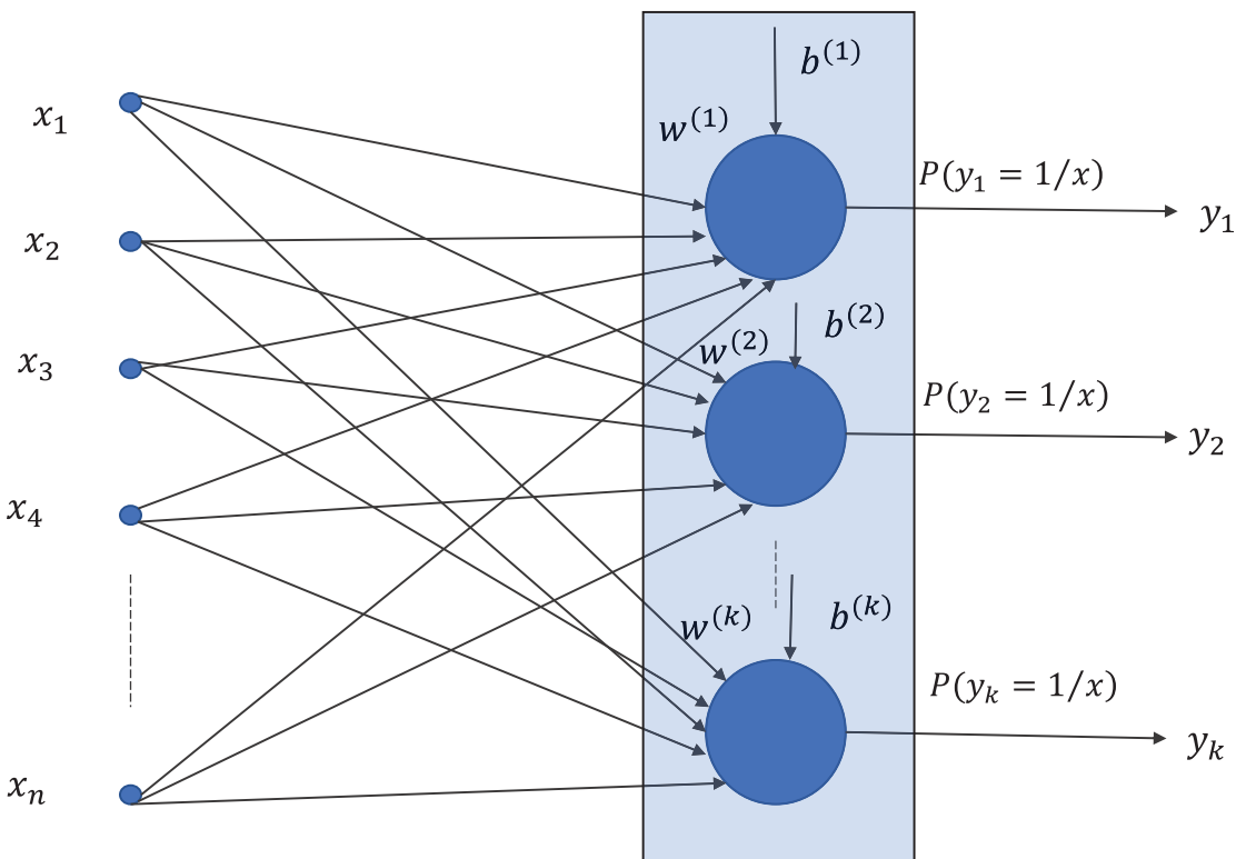
Figure 2-12. SoftMax activation function
