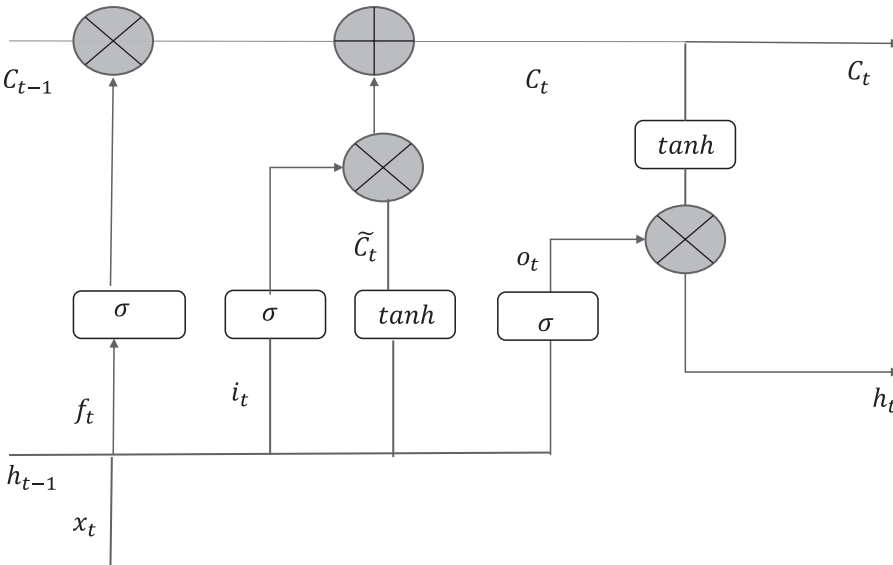
Figure 4-12. LSTM architecture
