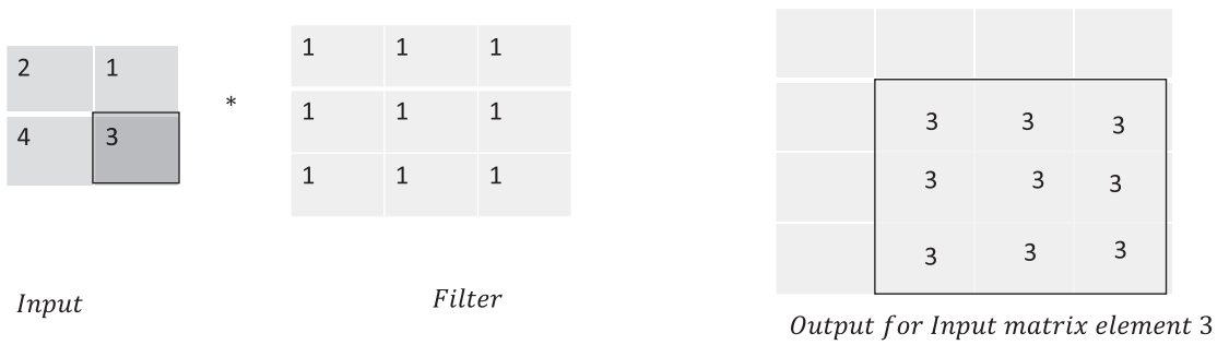
Figure 6-13b. Transpose convolution for upsampling
