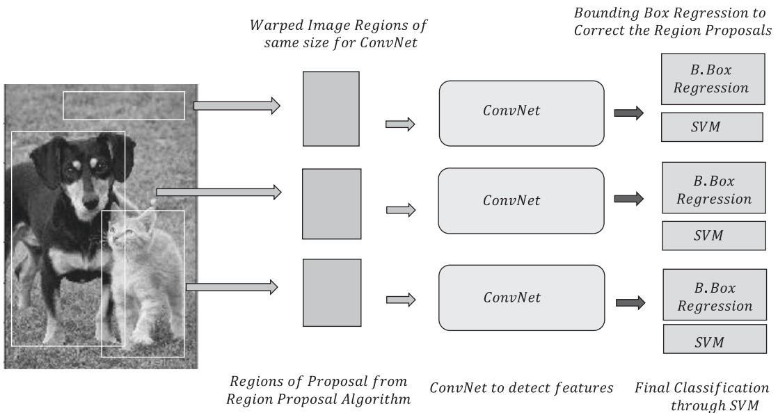
Figure 6-18. R-CNN network
