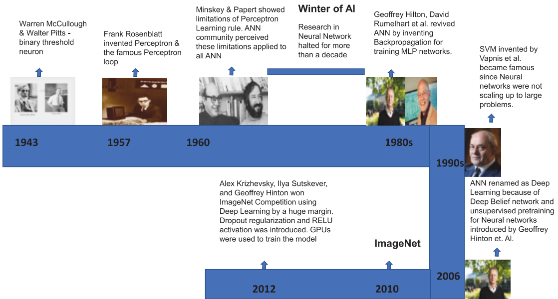
Figure 2-3. Evolution of artificial neural networks
