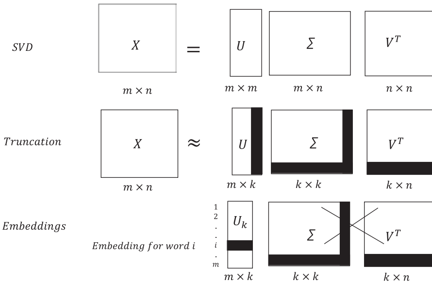
Figure 4-7. Extraction of word embeddings through SVD of word co-occurrence matrix
