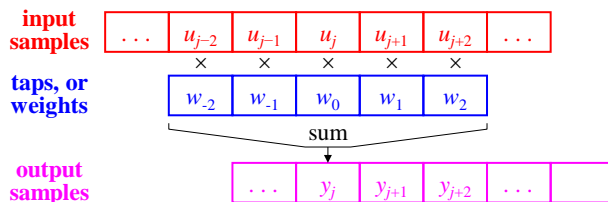
Figure 10.6 Example of a 5-tap FIR filter.
