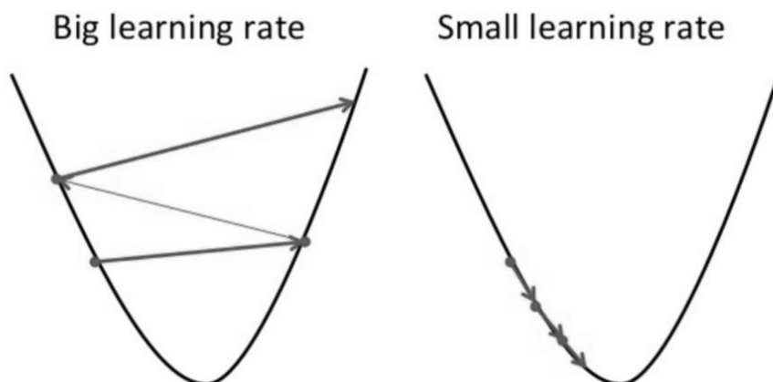
Fig.2 Gradient Descent
