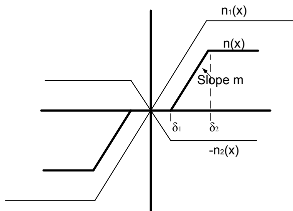
Figure 9.1 Nonlinearity and its synthesis from two ideal saturation characteristics.
