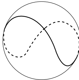
Figure 4.15: Tennis ball
