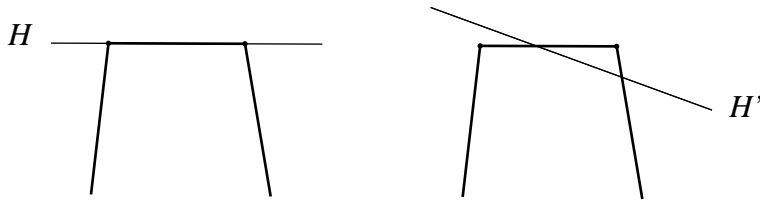
Figure 4.10: Multiplicity 2
