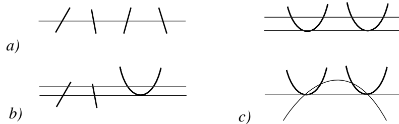
Figure 2.3: Total multiplicity 4
