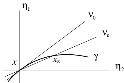
Figure 5.2: Bompiani construction
