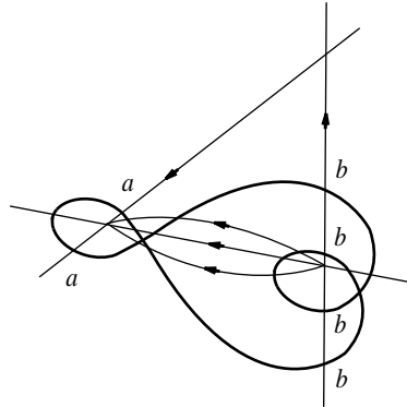
Figure 6.1: aabbbb
