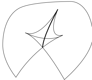
Figure 1.4: Swallow tail
