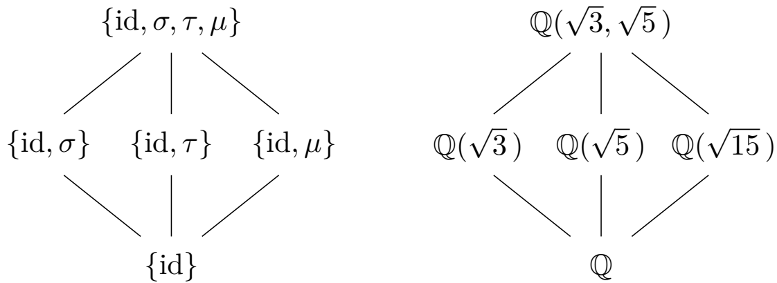
Figure 23.22 G(\mathbb{Q}(\sqrt{3}, \sqrt{5})/\mathbb{Q})
