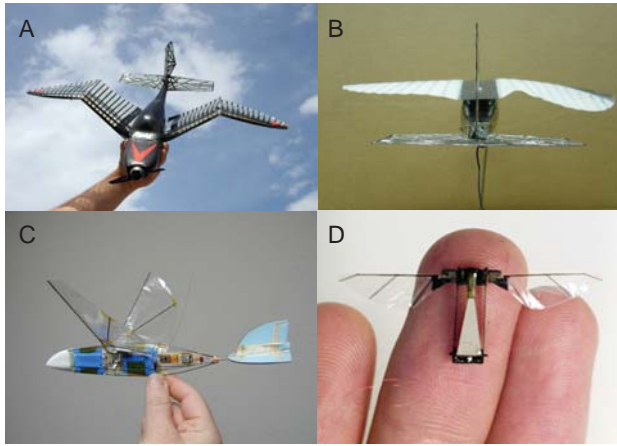
Fig. 5 | Examples of successful morphing and flapping micro air vehicles. (A) Gull-like variable wing dihedral for enhanced stability versus maneuverability (Lind et al. , 2004). (B) Bird-like wing twist for enhanced roll-performance (Lind et al. , 2004). (C) Insect-like flapping wings that generate both lift and thrust (Pornsirak et al. , 2001) (D) Prototype robotic fly that can take-off guided by wires (Wood, 2008).
