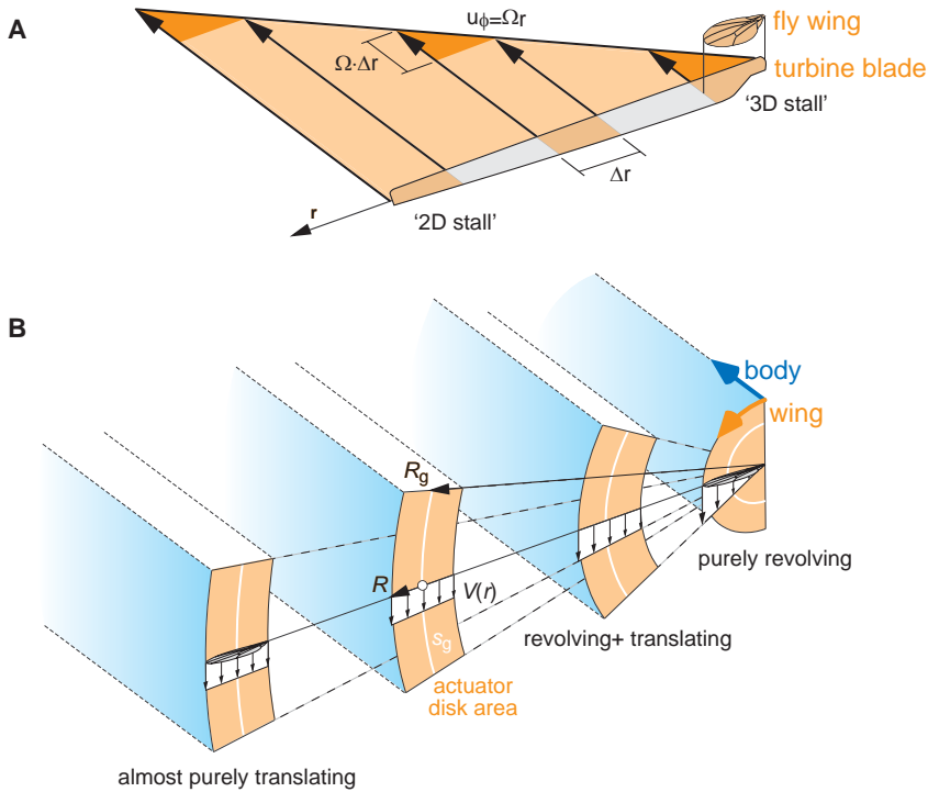
Fig. 9 | Is there an analogy between the influence of rotational accelerations on the stall characteristics of wind turbines and flapping fly wings? (A) Slender wings, such as wind turbine blades, have been found to possess distinctly different stall mechanisms near the root, for r/c < 3 where they stall locally 'three-dimensional', and near the tip, where they stall locally 'two-dimensional'. Fly wings are much less slender than wind turbine blades, therefore their whole wing is 'submerged' in the region of 'three-dimensional stall'. Clearly the circular path (in the stroke plane) of outward wing sections become progressively less curved compared to chord length. We illustrated how the local 'rotational component' of the radial speed component \Omega \cdot \Delta r becomes less and less important towards the tip compared to the 'linear component' of radial speed \Omega \cdot r . By taking \Delta r = c we find that the ratio of 'linear component' over 'rotational component' of radial speed is exactly r/c . (B) Based on the observations in (A) we designed flapping wing kinematics that allow us to change the relative importance of rotational accelerations R/c for a fly wing, which has a constant geometric slenderness. We achieved such a gradual transition from a linear velocity distribution to a constant velocity over the wing by gradually sticking the fly wing more outward on an extension rod between the wing and its joint. In this we keep the stroke amplitude 'actuator disk' areas swept by the wing in the stroke plane constant (orange) while it travels forward (blue). It can be demonstrated that a constant actuator disk area corresponds with a nearly constant stroke amplitude along the path s_g at the radius of gyration R_g . The relative curvature of the wing sections path with respect to its chord length is again measured by R/c the single wing aspect ratio. Graphically we can directly infer that the paths traveled at more outward radii are much less curved and therefore the corresponding three-dimensional rotational accelerations will diminish.
