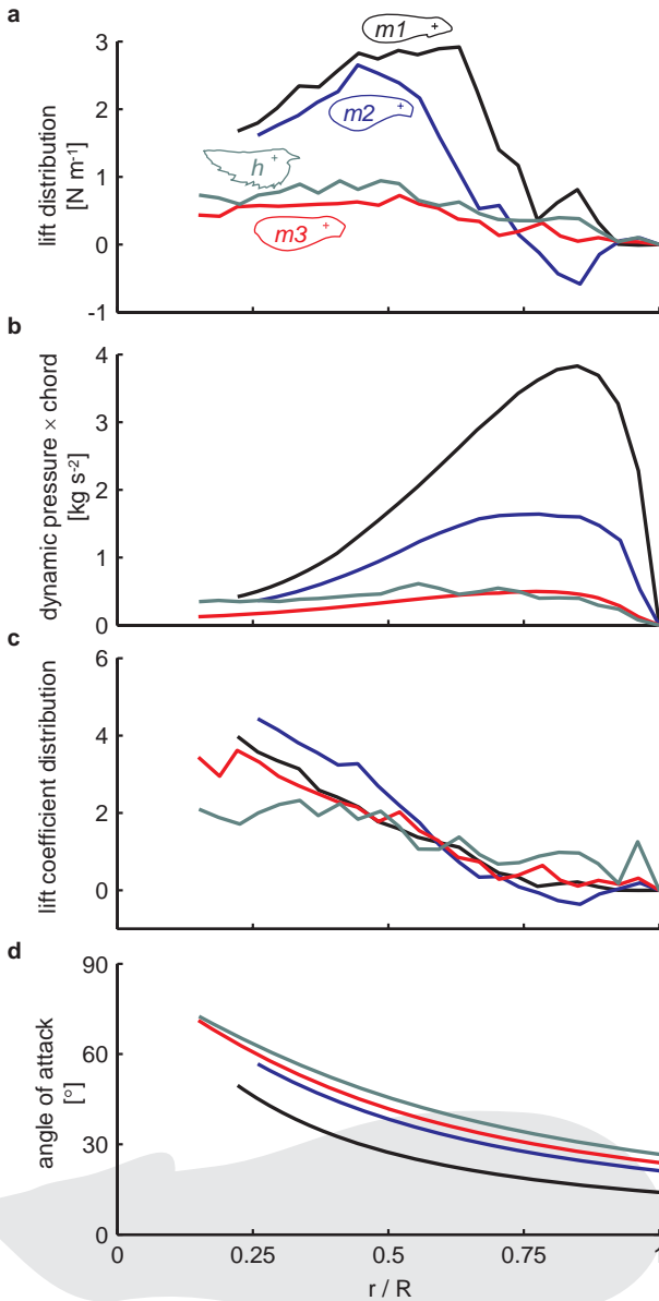
Figure 4 | The LEV induces exceptional high local lift coefficients near the wings base. a, Spanwise lift distribution. The wing's sectional lift is particularly low near the wing tip due to the presence of the tip vortex ( r , local radius; R , wingtip radius; seed code, Fig. 1b). b, Product of sectional dynamic pressure and chord length. c, The wing's lift sectional coefficient ( a divided by b ), peaks near the wing's base (where a LEV is present) and it is minimal at the tip. d, The distribution of angle of attack with span. The high lift coefficients near the base of the wing ( c ) and the corresponding LEV result from the extremely high local angles of attack, well beyond 30^\circ .
