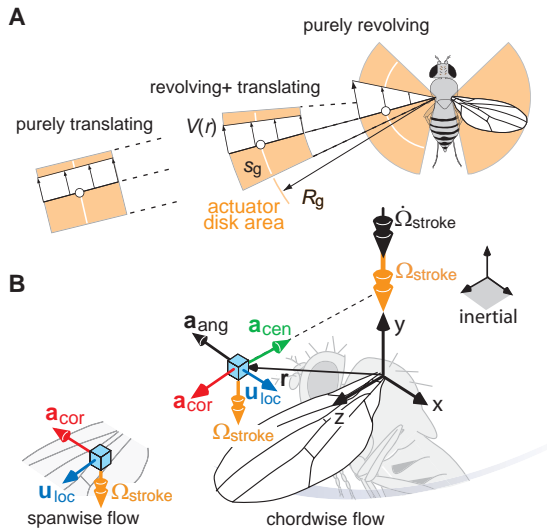
Fig. 3 | Theoretical and experimental approach. (A) Framework used to analyze fluid accelerations on translating and revolving wings. The area of the actuator disk is constant within the model. R_g is the radius of gyration, s_g the number of chord lengths traveled at R_g during a full stroke, and V(r) is the velocity distribution along the wings radius r . (B) In the wing-bound frame, the fluid close to the wing experiences three accelerations due to the wing’s stroke kinematics: an angular acceleration \mathbf{a}_{\text{ang}} a centripetal acceleration \mathbf{a}_{\text{cen}} and a Coriolis acceleration \mathbf{a}_{\text{cor}} . Note that \mathbf{u}_{\text{loc}} is the local velocity in the wing-bound frame, \Omega_{\text{stroke}} is the angular velocity due to stroke, and \dot{\Omega}_{\text{stroke}} is the angular acceleration due to stroke.
