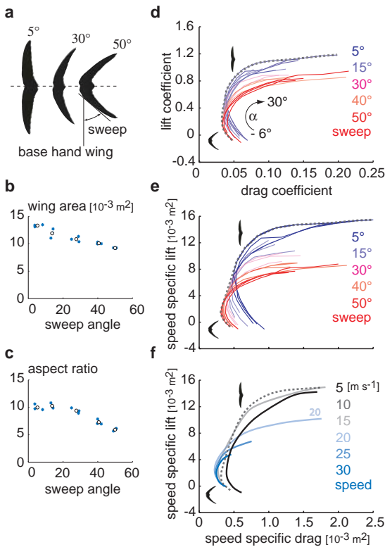
Figure 2 | Morphing swift wings can generate higher lift and lower drag than wings with a fixed geometry.
