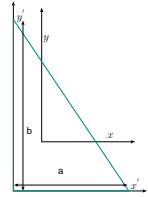
Fig. -3.13. Product of inertia for triangle.
