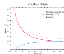
Fig. -1.25. The raising height as a function of the radii.
