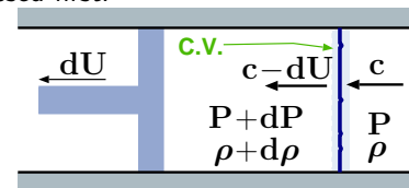
Fig. -11.2. Stationary sound wave and gas moves relative to the pulse.
