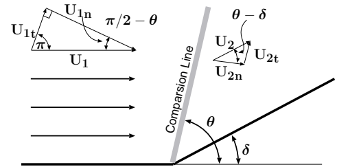
Fig. -12.3. A typical oblique shock schematic.
