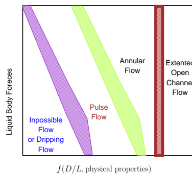
Fig. -13.10. Counter-flow in vertical tubes map.
