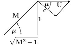
Fig. -12.22. The angles of the Mach line triangle.
