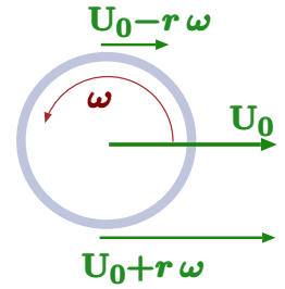
Fig. -10.17. Schematic to explain Magnus’s effect.
