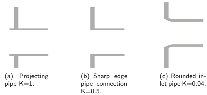
Fig. -7.4. Typical resistance for selected outlet configuration.
