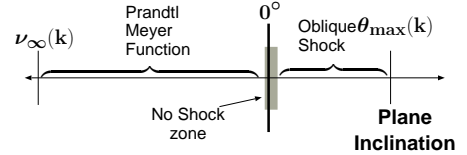
Fig. -12.2. The regions where oblique shock or Prandtl-Meyer function exist. Notice that both have a maximum point and a "no solution" zone, which is around zero. However, Prandtl-Meyer function approaches closer to a zero deflection angle.
