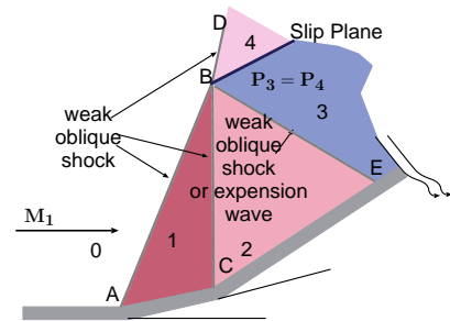
Fig. -12.16. Schematic of two angles turn with two weak shocks.
