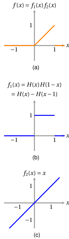
Figure 7.7: Composition of f(x) = f_1(x)f_2(x) .
