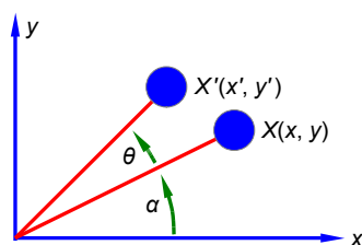
Figure 5.16: rotation in a plane.
