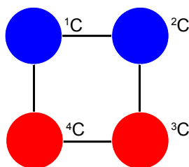
Figure 6.21: \psi_3 SOMO of cyclobutadiene looking down on the 2p AOs.
