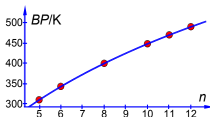
Figure 2.14: boiling points of n -alkanes.
