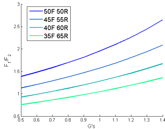
Figure 24: The impact of the front rear weight distribution on the normal force ratio during deceleration.
