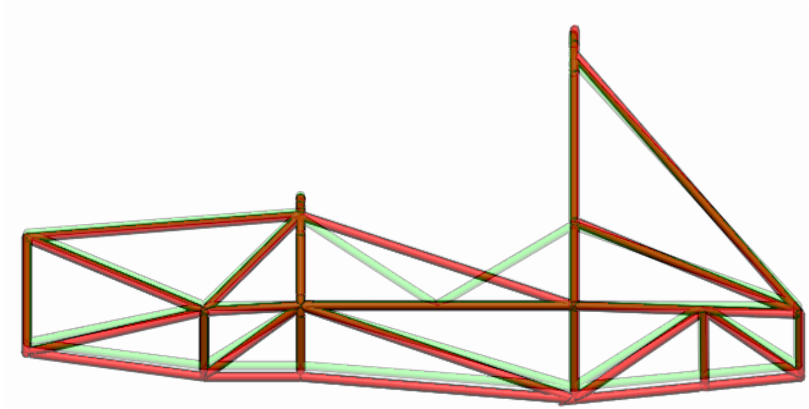
Figure 6: Iteration 1 chassis with iteration 2 chassis (Red) overlaid on top
