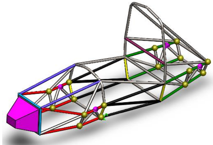
Figure 14: : Locations of suspension mounting locations, the Golden dots indicate the A-arm mounting locations, the pink dots indicate the shock mounting locations.
