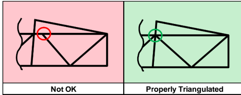
Figure 39: Node to Node Triangulation.
