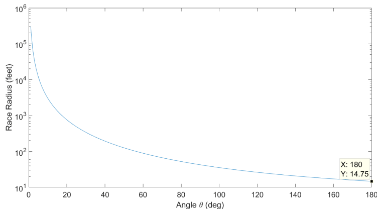
Figure 29: The race radius as a function of the turn angle \theta
