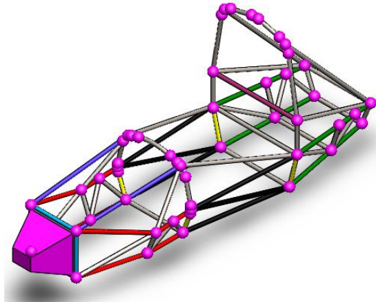
Figure 33: Frame joints, indicated by the pink dots, auto created by SolidWorks).
