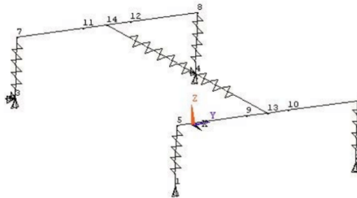
Figure 19: The simplified compliant spring and frame model presented by Riley and George [5]. Here the horizontal spring from node 13 to 14 represents the compliance of the frame while the remaining represent the spring rate of the suspension.
