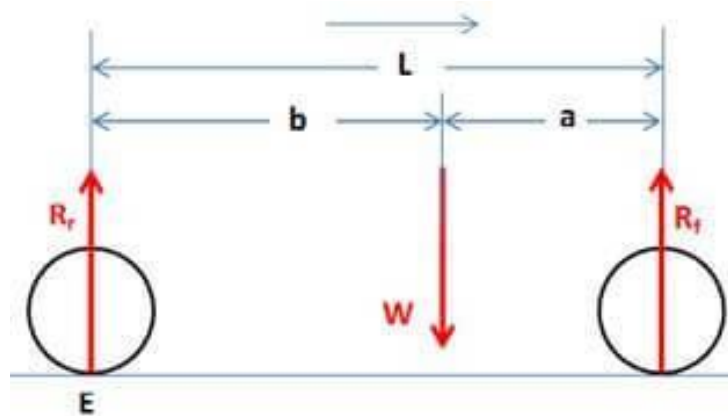
Figure 36: Free-body diagram of the force on a car as viewed from the side.
