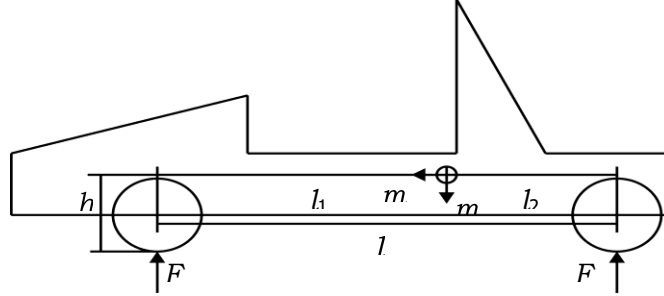
Figure 23: Wheel load schematic under the braking process.
