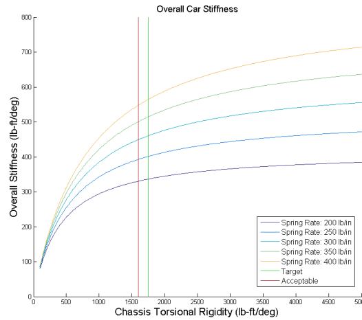
Figure 22: The overall car stiffness as a function of the chassis' stiffness for several different spring rates.
