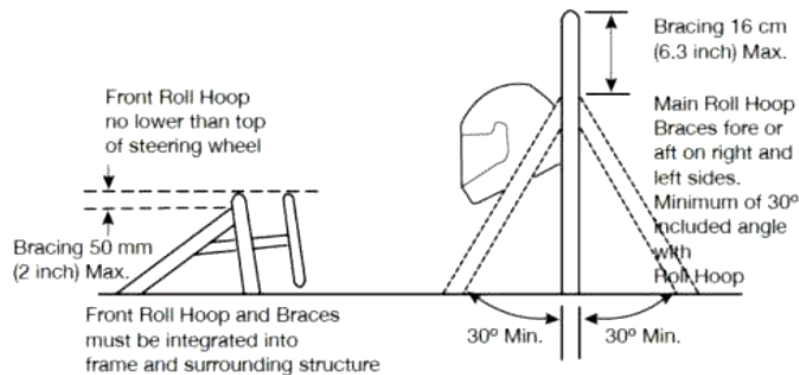
Figure 40: Main Roll Hoop Rules
