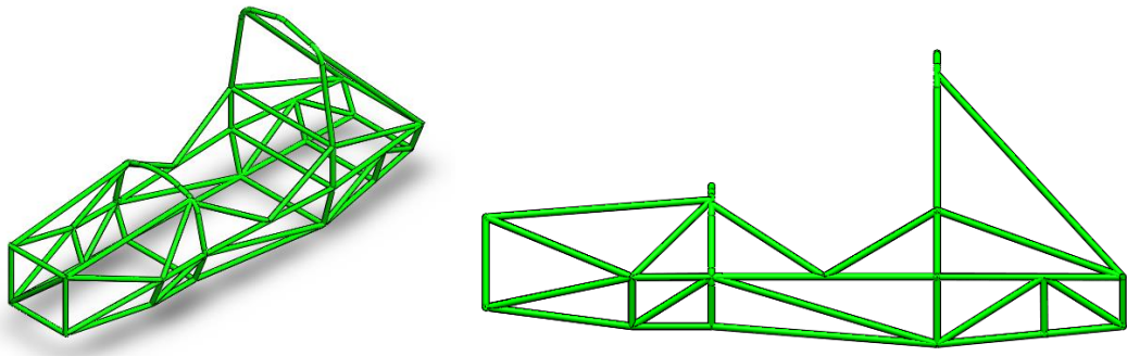
Figure 3: Iteration 1 isometric (left) and side view (right).
