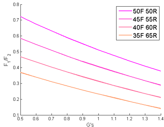
Figure 25: The impact of the front rear weight distribution on the normal force ratio during acceleration.
