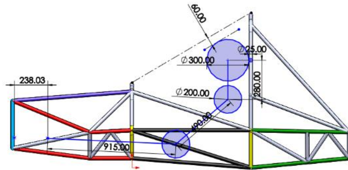
Figure 12: Rule T3.10 states that the top of the person's helmet must be no closer than 2 inches, and the back of the head no closer than two inches to the specified lines.
