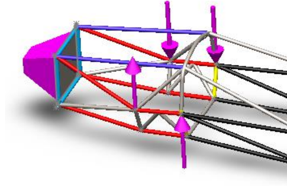
Figure 35: Various loads applied in the FEA tests.
