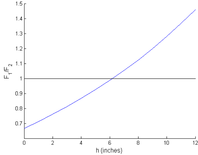
Figure 26: The weight distribution ratio plotted as a function of the center of gravity's vertical height. The black horizontal line indicated the ideal ratio of 1.
