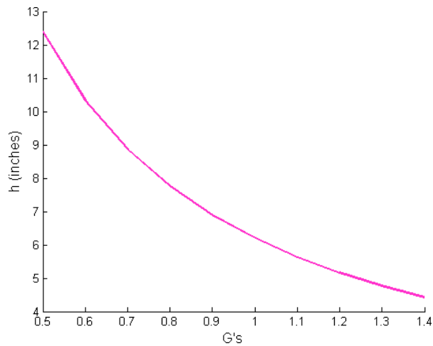
Figure 27: The ideal height of the center of gravity for even front rear weight distribution as a function of deceleration.
