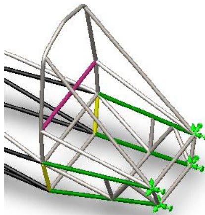
Figure 34: Fixtures applied to the rear box.
