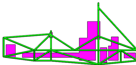
Figure 4: Iteration 1 centre of mass calculation, based on approximate weights, volumes, and positions, see Appendix F.2 for details.
