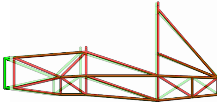
Figure 8: Iteration 2 chassis with iteration 3 chassis (red) overlaid on top.
