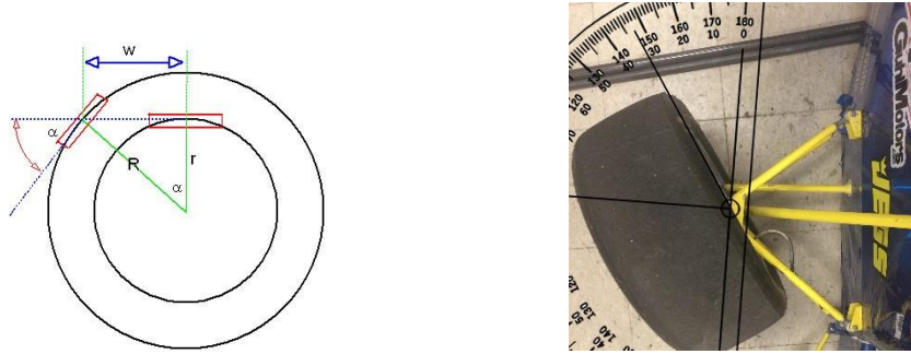
Figure 30: Geometry of a fixed back wheel and a front wheel turning at angle \alpha (left), and a photo of the angle on the 2019 chassis at max steer angle of 33 degrees (right).
