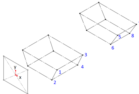
Figure 2: Node ID layout of the chassis frame. Also note that the origin is defined at the centre of the front impact attenuator
