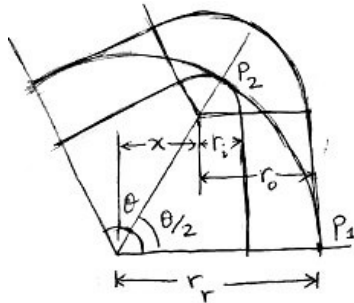
Figure 28: Diagram of the outer, inner, and race radii r_o , r_i , and r_r respectively.
