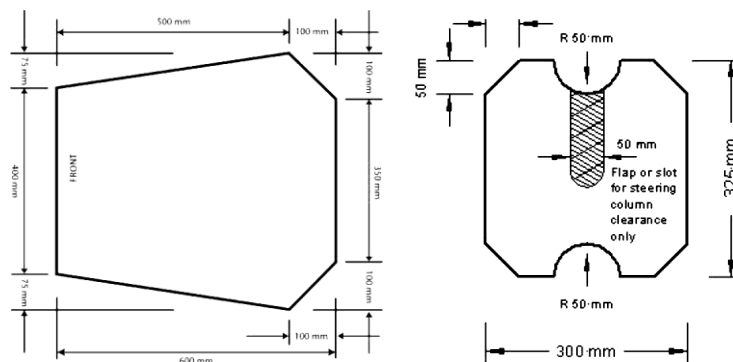
Figure 42: Cockpit Template (Left), Foot well template (Right).
