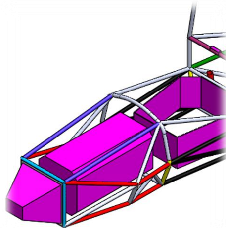
Figure 13: Rules T4.1 and T4.2 state that specified templates must be passed through the chassis to ensure that there is ample room for the driver to get in and out.
