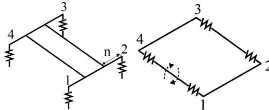
Figure 20: Simplified model of a car's wheel rates attached to a rigid chassis. (a) represents the wheel rates as a set of translational springs and (b) represents the wheel rates as torsional springs directly attached to the chassis.
