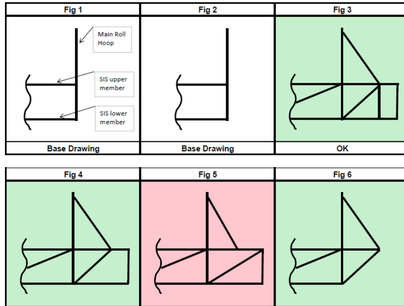
Figure 41: MRH Bracing Configuration
