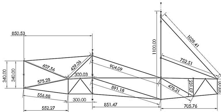
Figure 11: All Dimension sketch, see Appendix F.2 for details.
