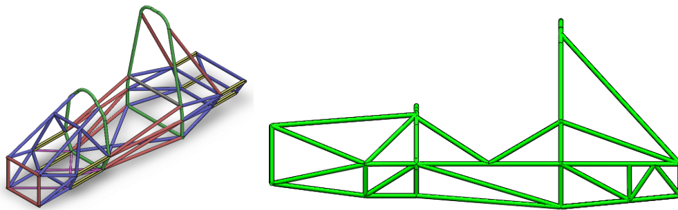
Figure 1: The two initial frame concepts created to start the iteration process.
