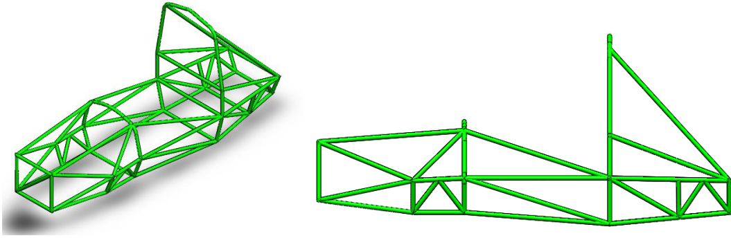
Figure 9: Iteration 4 isometric (left) and side view (right).
