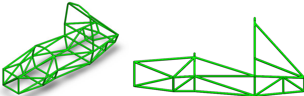
Figure 5: Iteration 2 isometric (left) and side view (right).
