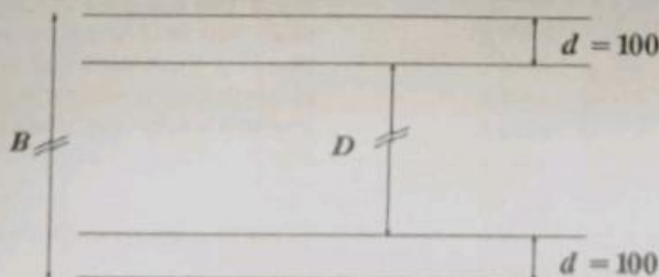
FIG. 5 ZONE FOR THE MEASUREMENT OF OPTICAL DISTORTION
