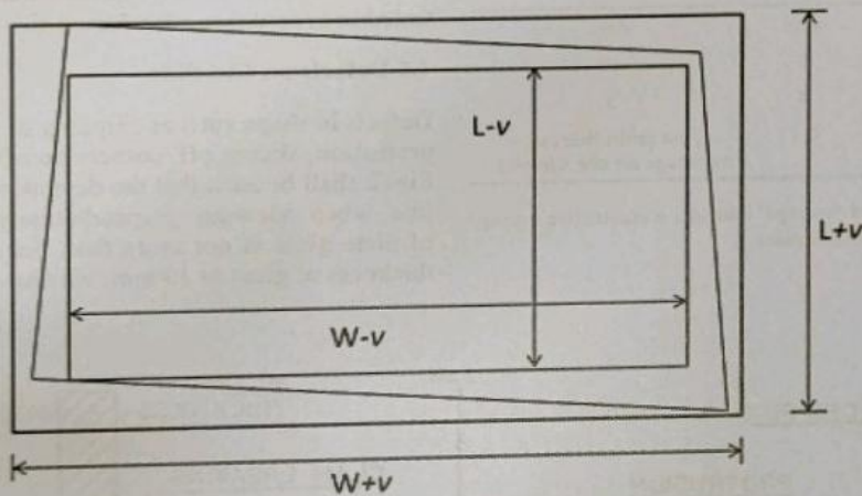
FIG. 1 TOLERANCE LIMITS FOR DIMENSIONS OF RECTANGULAR PANES
