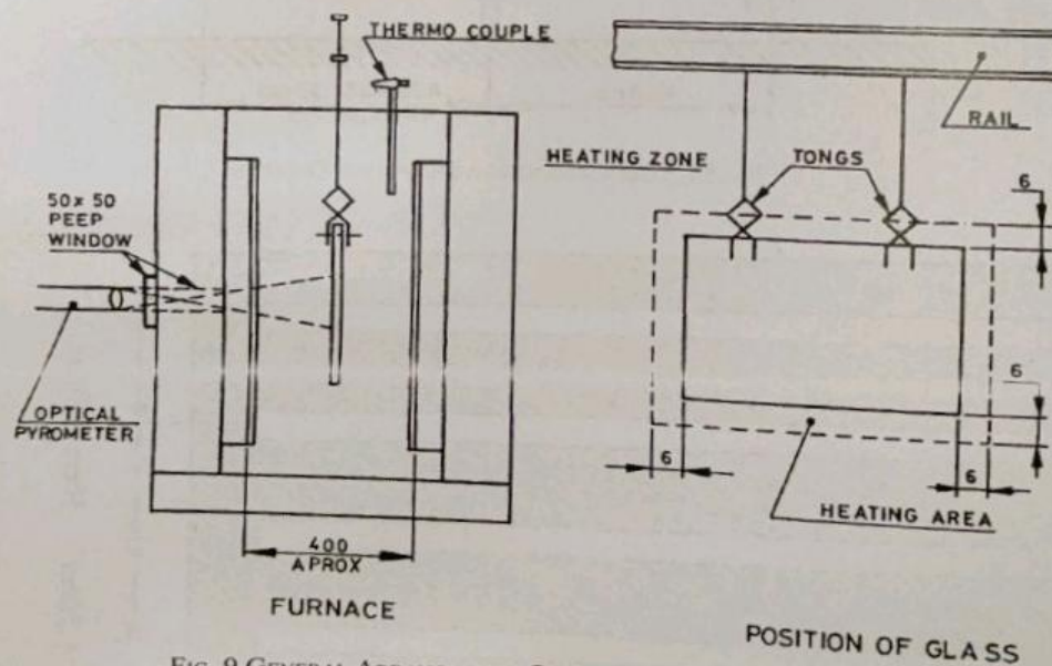
FIG. 9 GENERAL ARRANGEMENT OF ELECTRIC HEATING FURNACE
