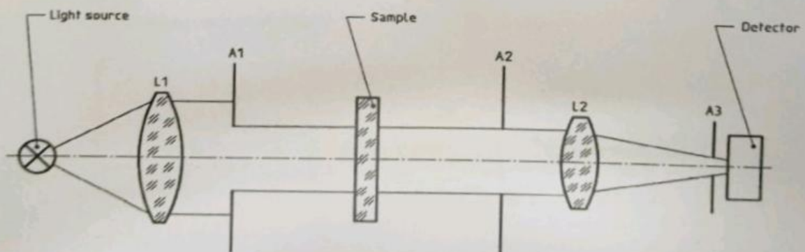
FIG. 3 MEASUREMENT OF LIGHT TRANSMITTANCE USING STANDARD ILLUMINANT
