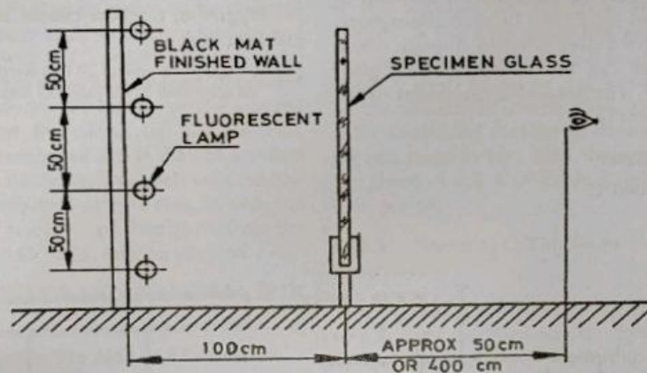
FIG.8A ARRANGEMENT FOR DETECTING DEFECTS
