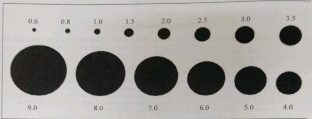
FIG. 7 EXAMPLE OF DISTORTION GAUGE WITH PRINTED BLACK SPOTS
