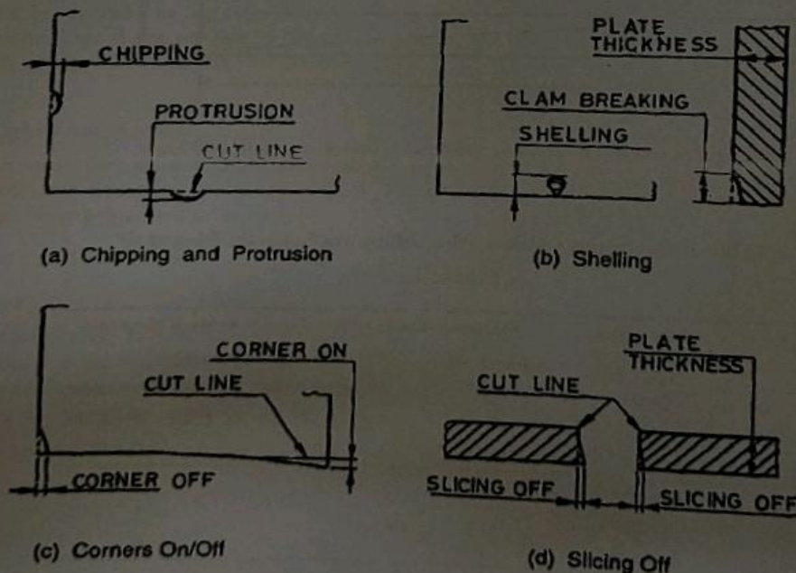
FIG. 2 DEFECTS ON CUT SIDE
