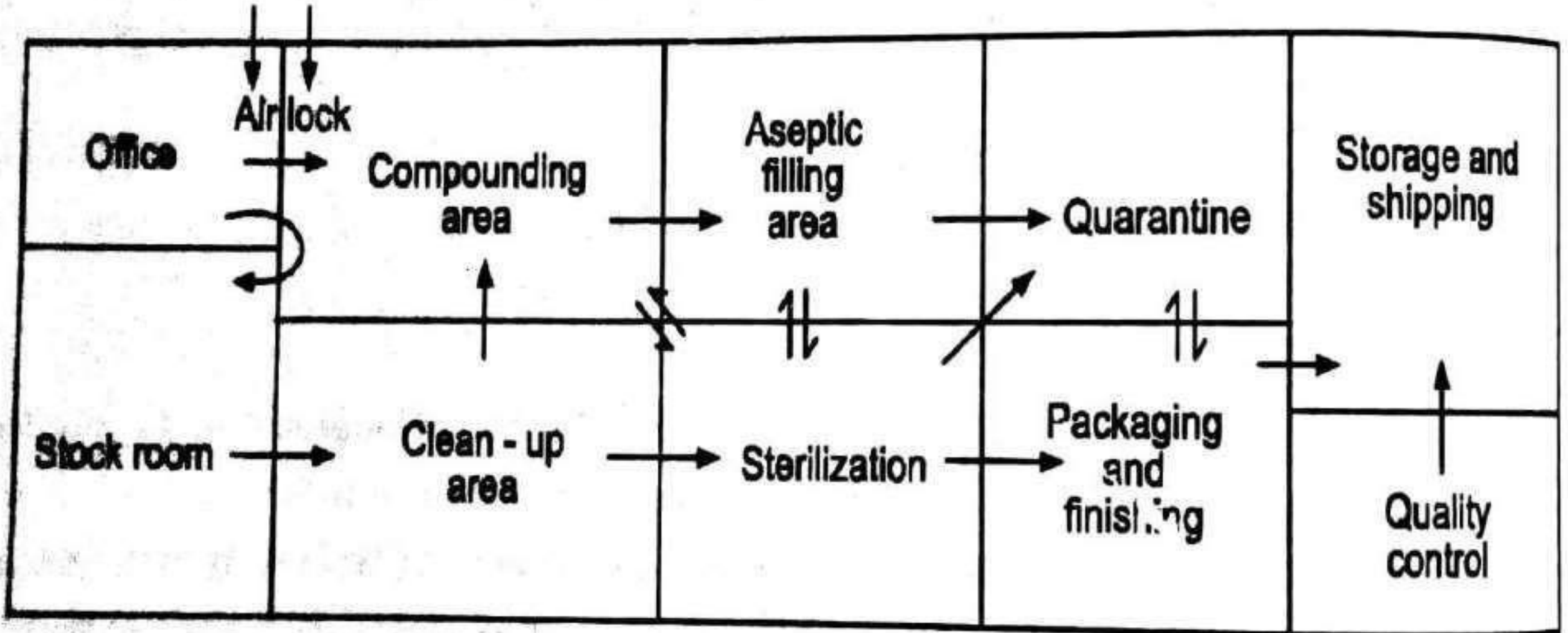
Fig. 18.1 : Flow diagram of aseptic area
