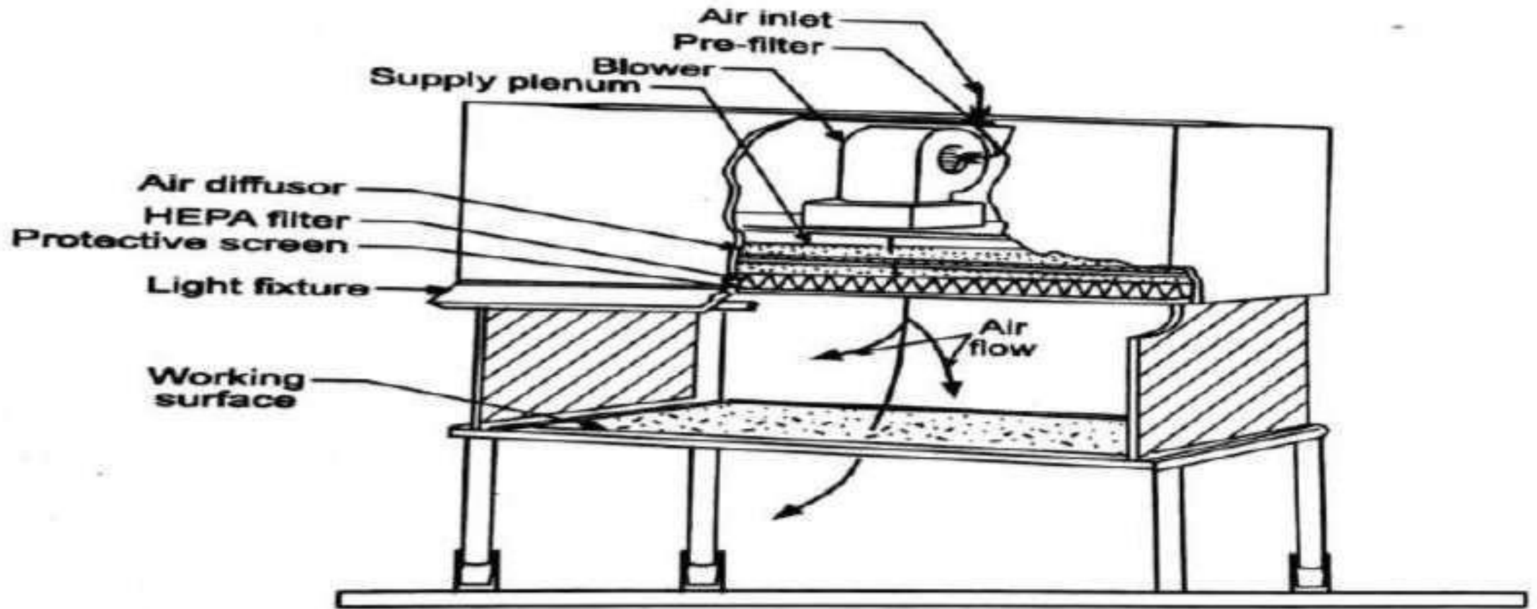
Fig. 18.2 : Vertical laminar air flow bench
