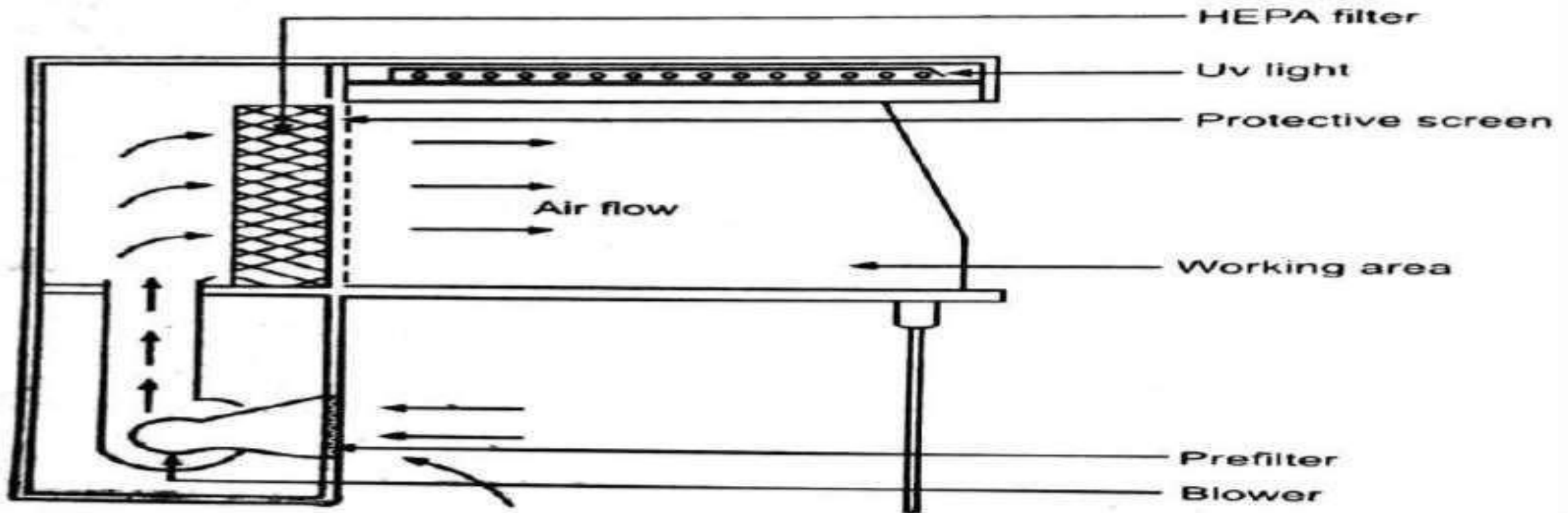
Fig 18.4 : Direction of air flow in a horizontal laminar air flow
