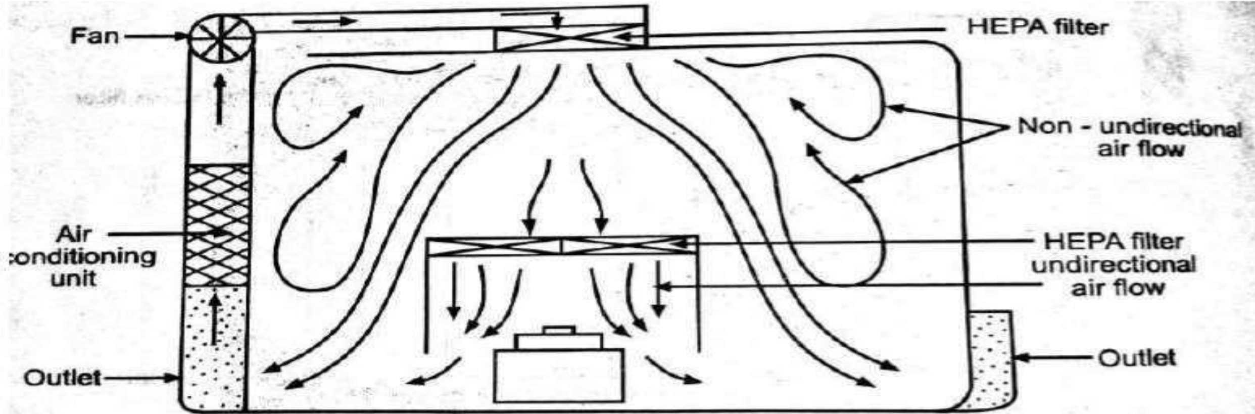
Fig. 18.7 : Combined airflow pattern
