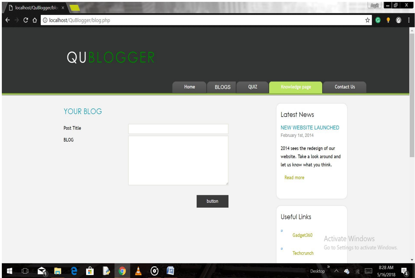
Fig 13: Write Blog
