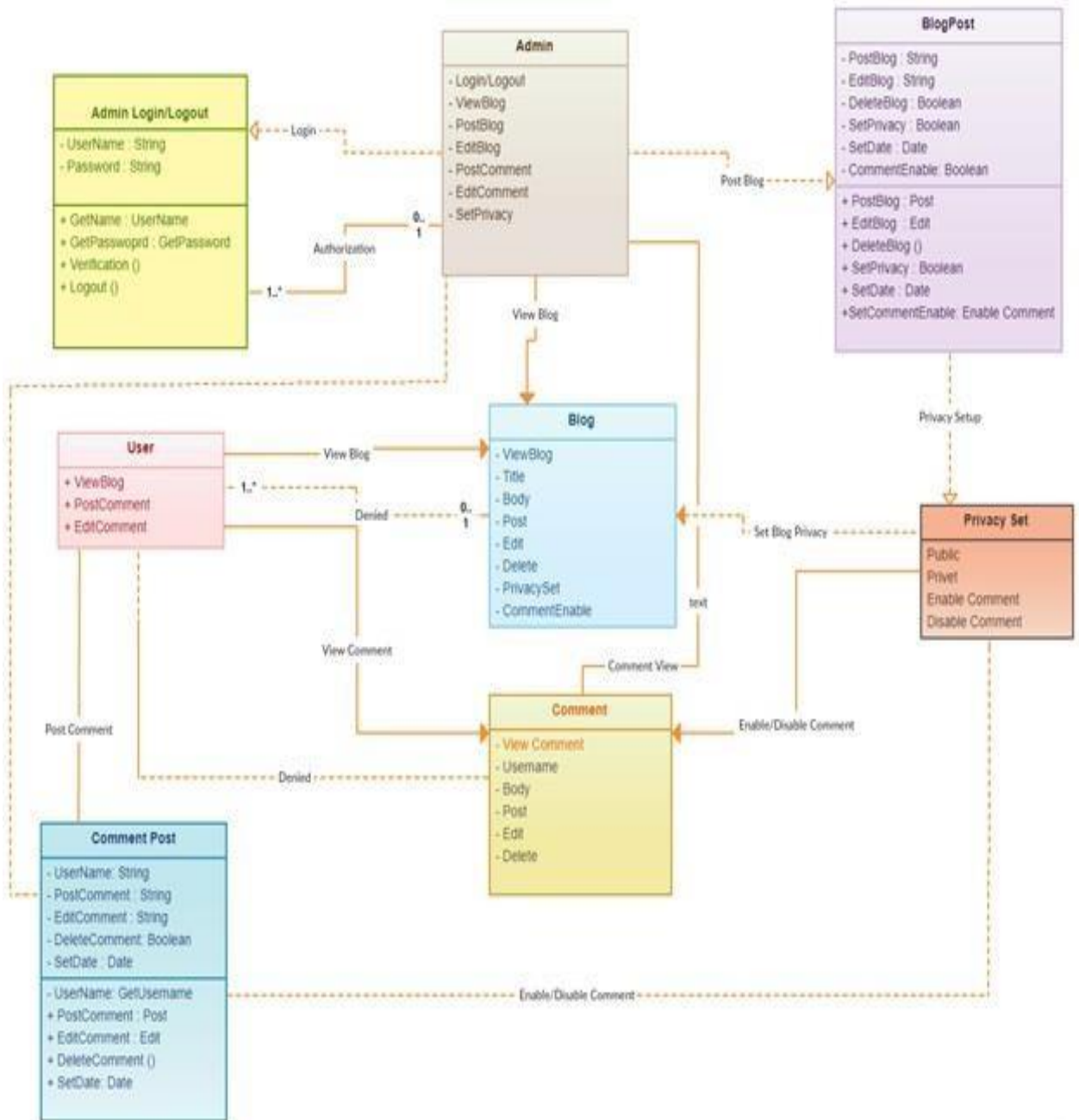
Fig 4: Class diagram
