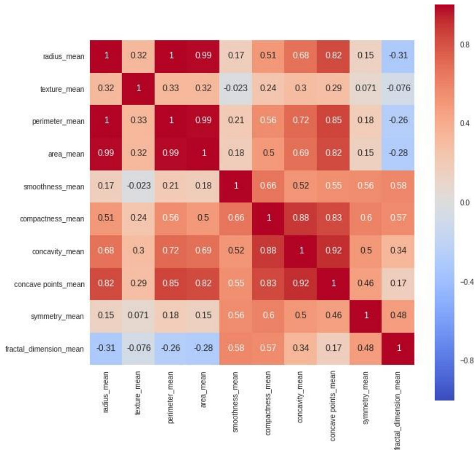
Figure 4: Heat Map
